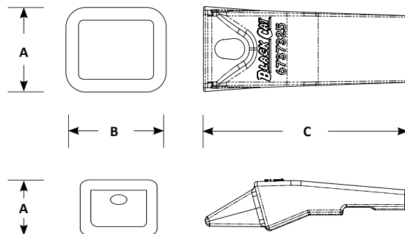
Bobcat® Tooth 6737325
