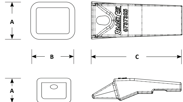
Bobcat® Tooth 6737325
